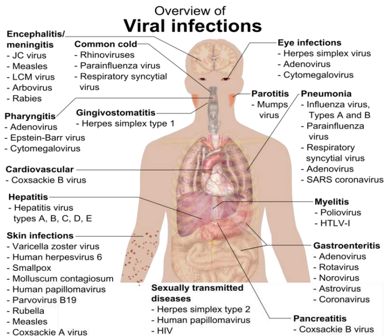
Figure 5: Overview of the main types of viral infection and the most notable species involved
