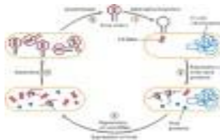
Figure 2: Viral Growth Cycles Are Classified as Lytic
