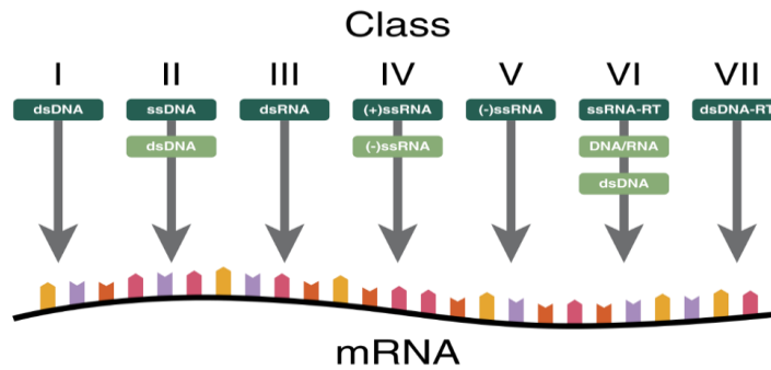
Figure 4: The Baltimore Classification of viruses is based on the method of viral mRNA synthesis
