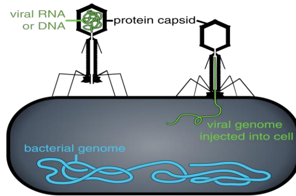
Figure 3: Some bacteriophages inject their genomes into bacterial cells
